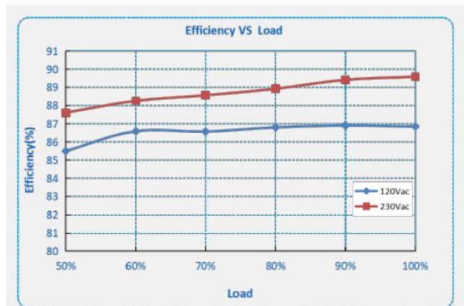
F1-060X-085 ( I_o=0.7A )
